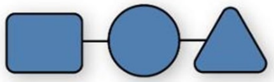
Figure 7-1: Diagram Shapes
